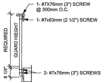
DETAIL (SB-7 DETAIL ED-1/ED-2) PICKET ATTACHMENT, TYPICAL
